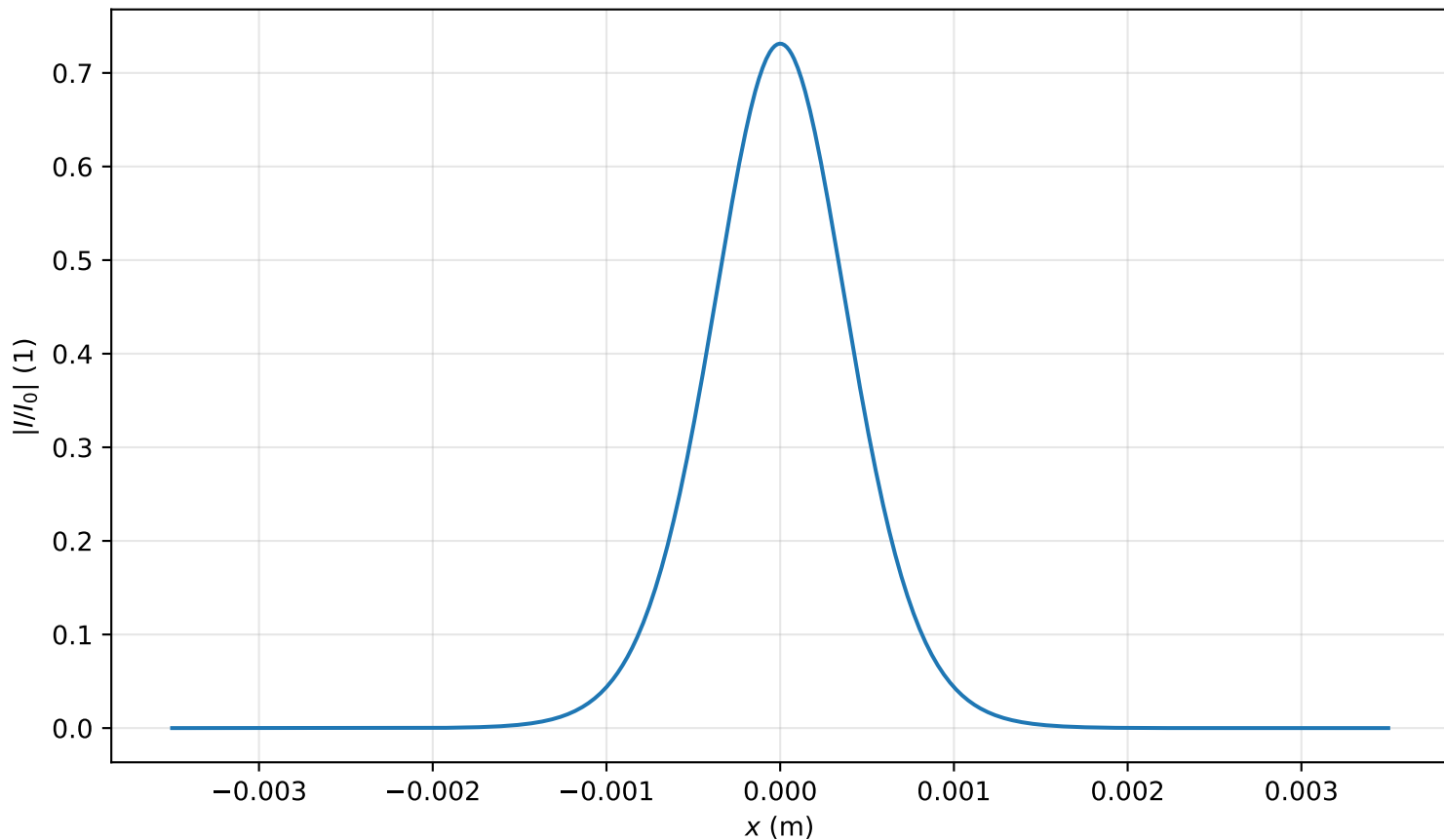
Intensity profile I(x, y = 0, z = 1.990m)/I_0 , Pin=0.4Pcr, artificial time
